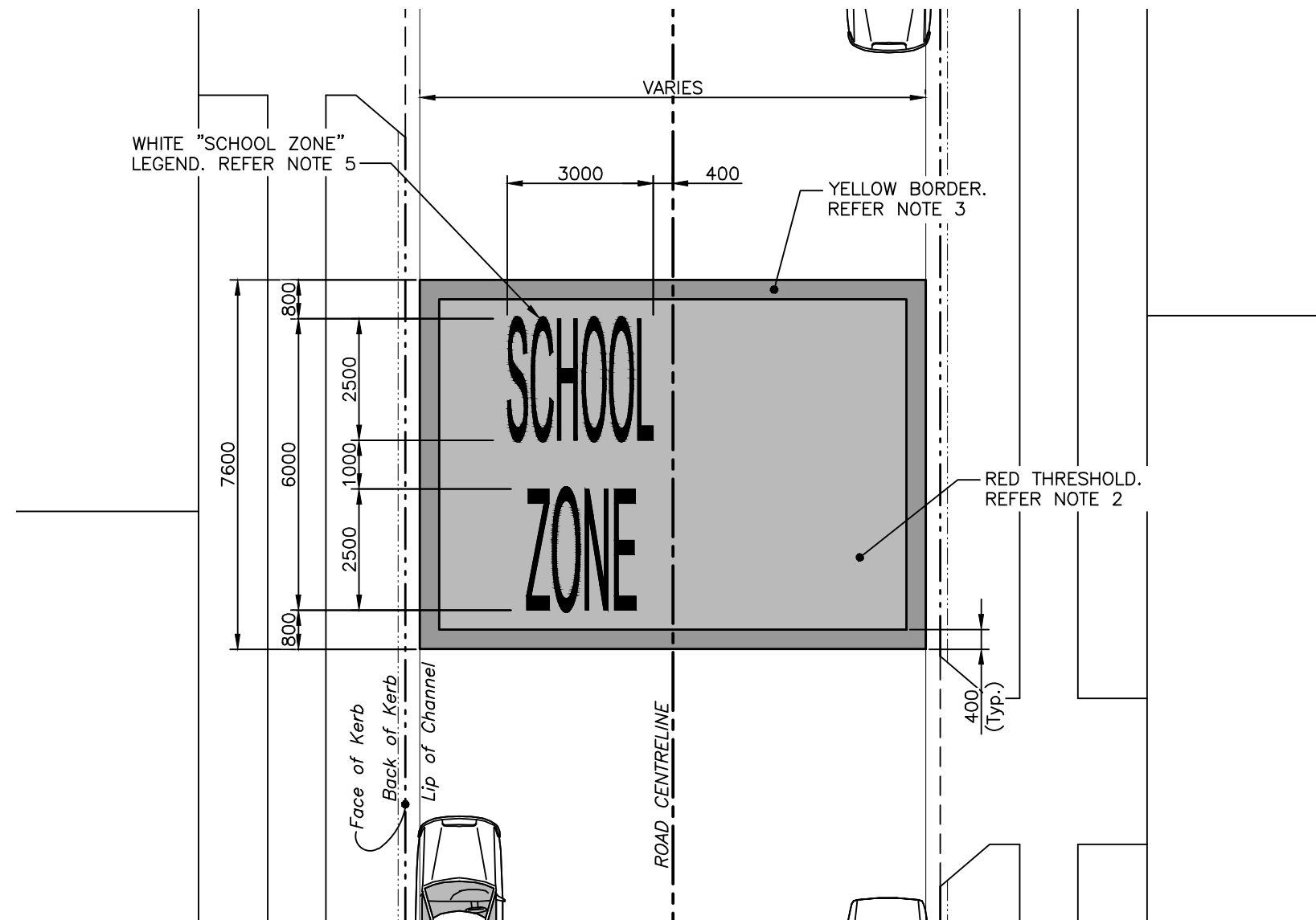
PLAN – PAVEMENT TREATMENT
