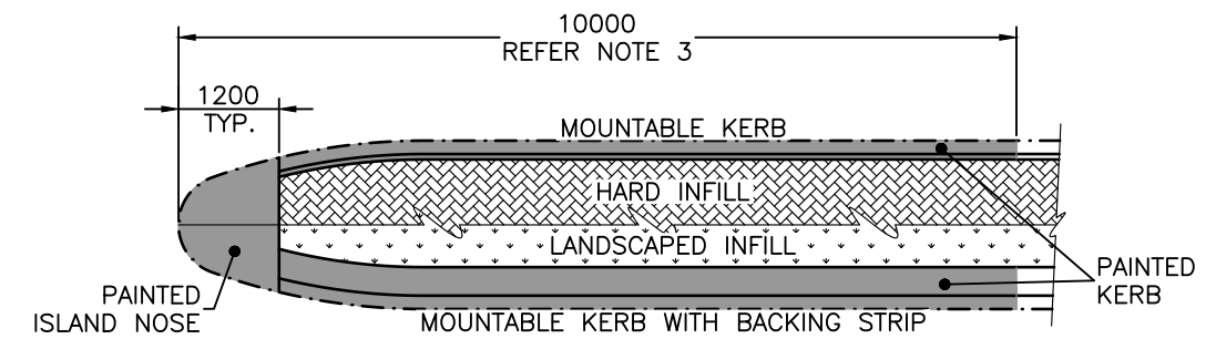
PAINTED MEDIAN/TRAFFIC ISLAND KERB (PAINT TOP AND FACE OF KERB)
