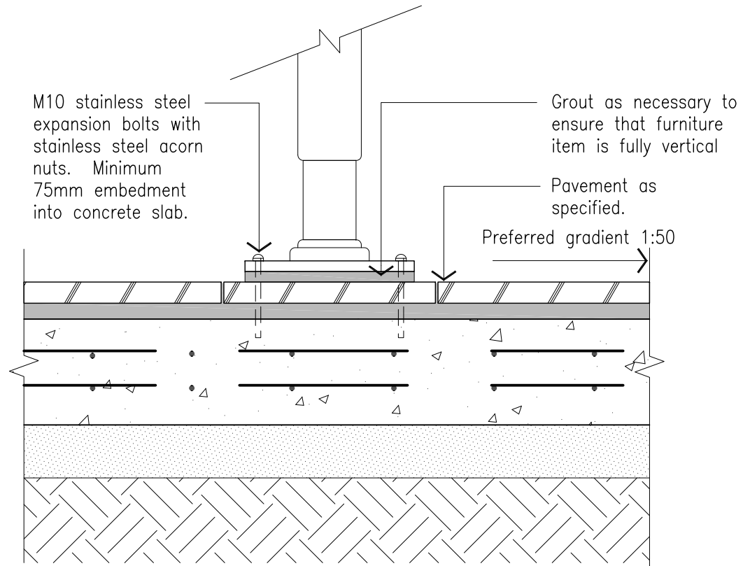
TYPICAL SECTION
