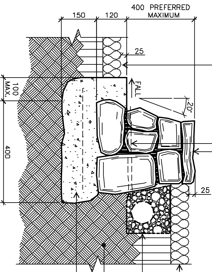
FREE STANDING STONE WALL – SECTION
